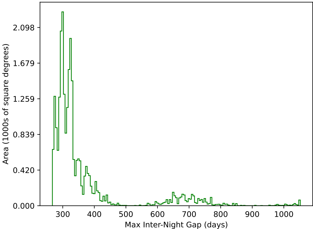
noroll_mjdp60_v3.4_10yrs All sky g band: Max Inter-Night Gap
