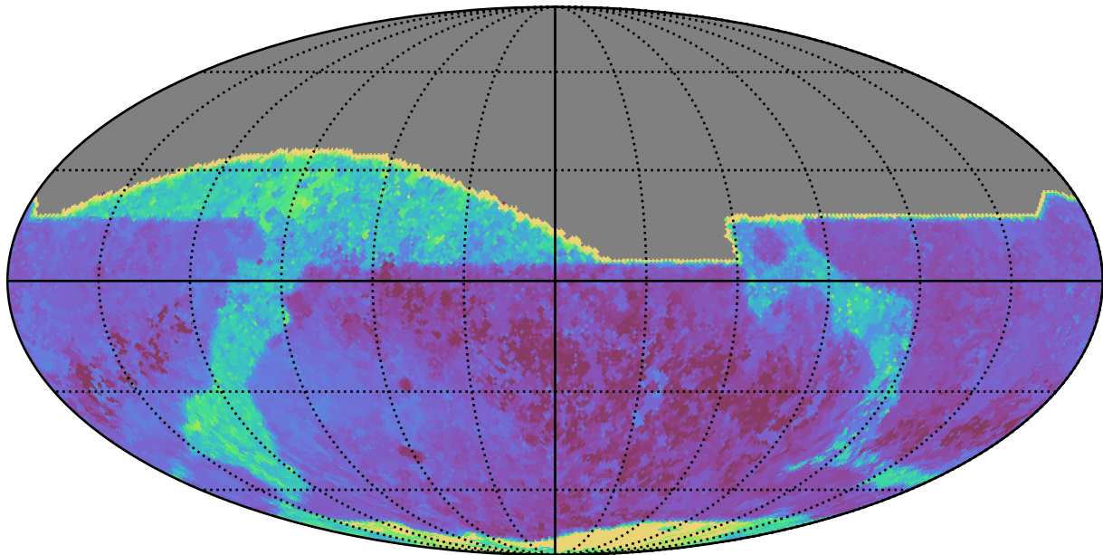
noroll_mjdp60_v3.4_10yrs All sky all bands: Max Inter-Night Gap
