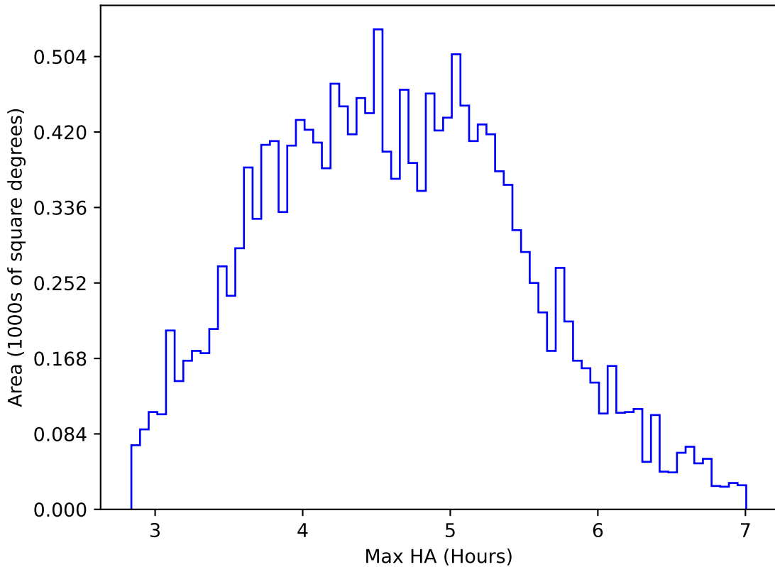
noroll_mjdp60_v3.4_10yrs WFD z band: Max HA
