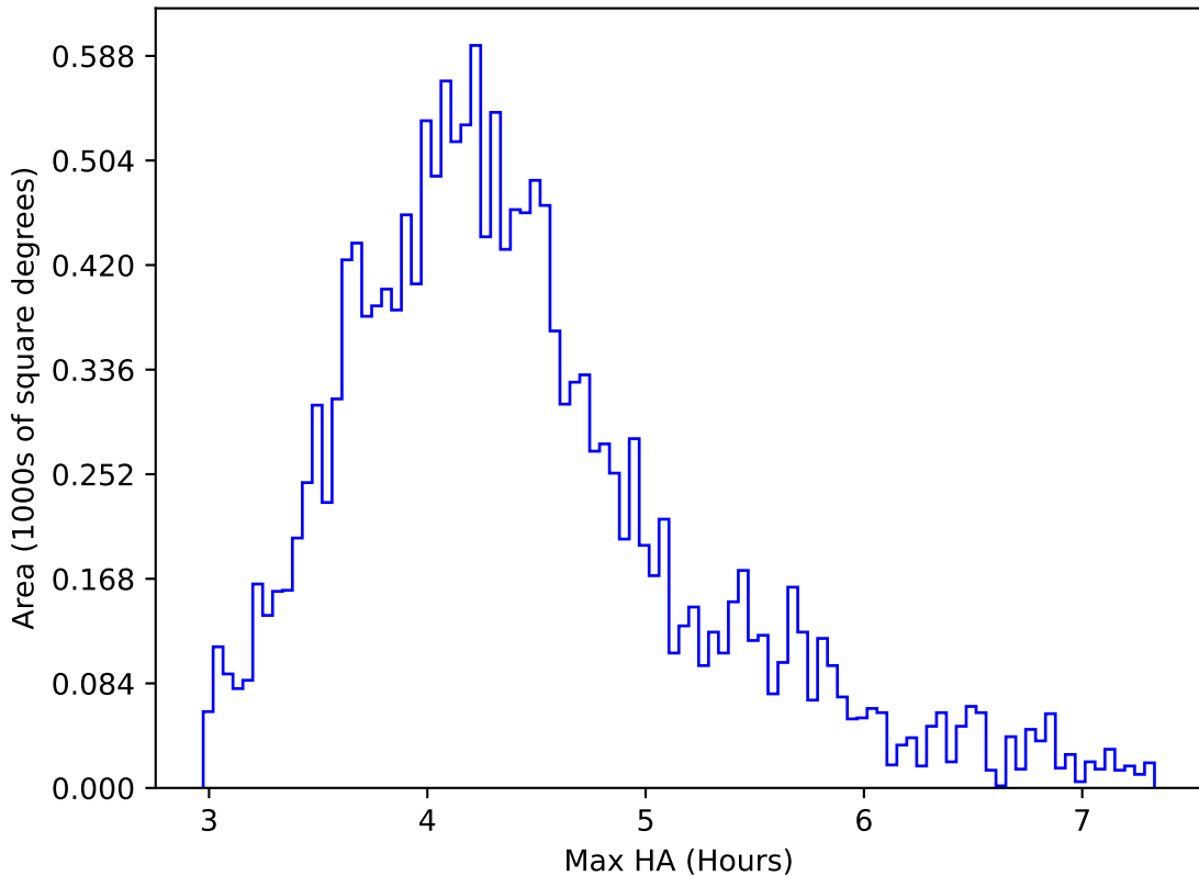
noroll_mjdp60_v3.4_10yrs WFD y band: Max HA
