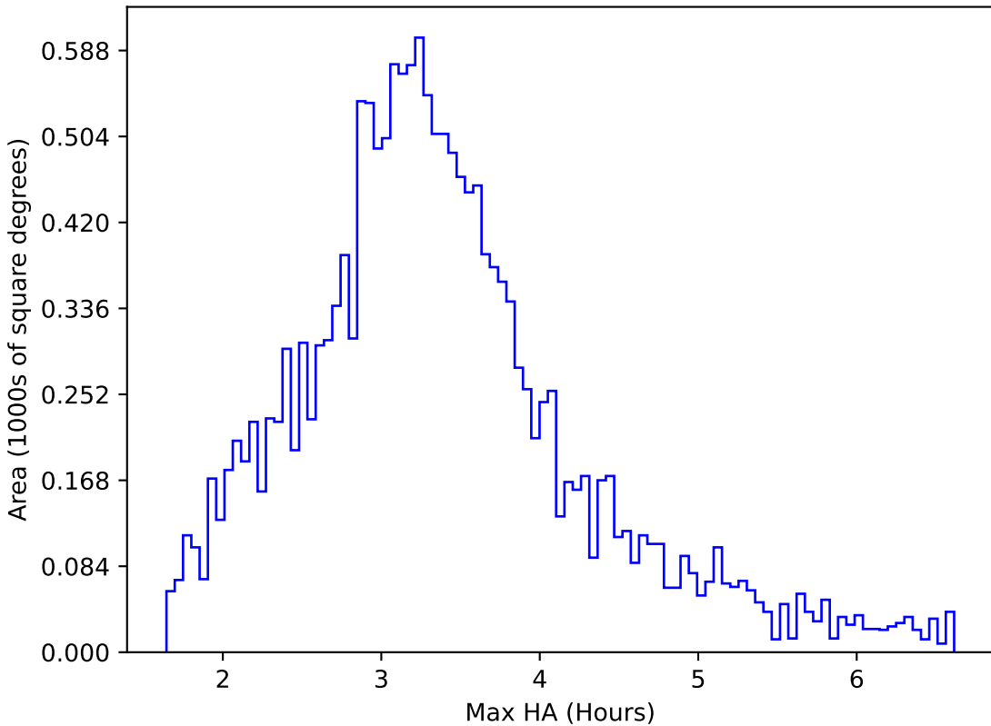
noroll_mjdp60_v3.4_10yrs WFD u band: Max HA
