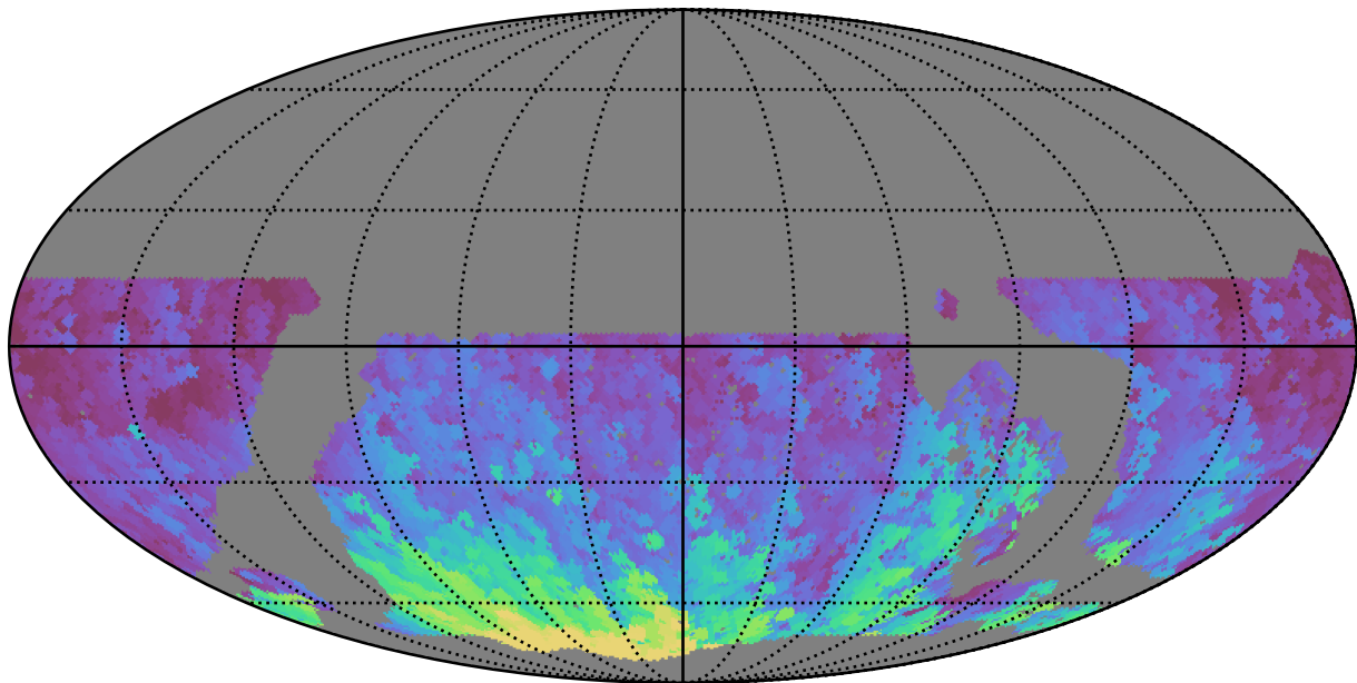
noroll_mjdp60_v3.4_10yrs WFD r band: Max HA
