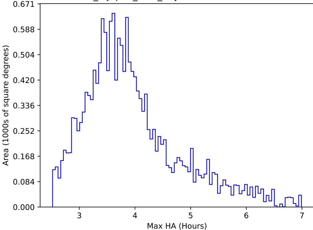
noroll_mjdp60_v3.4_10yrs WFD r band: Max HA
