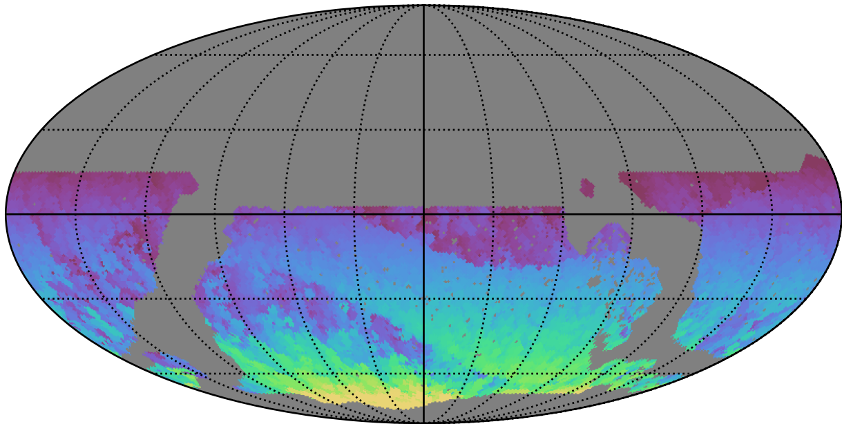
noroll_mjdp60_v3.4_10yrs WFD all bands: Max HA
