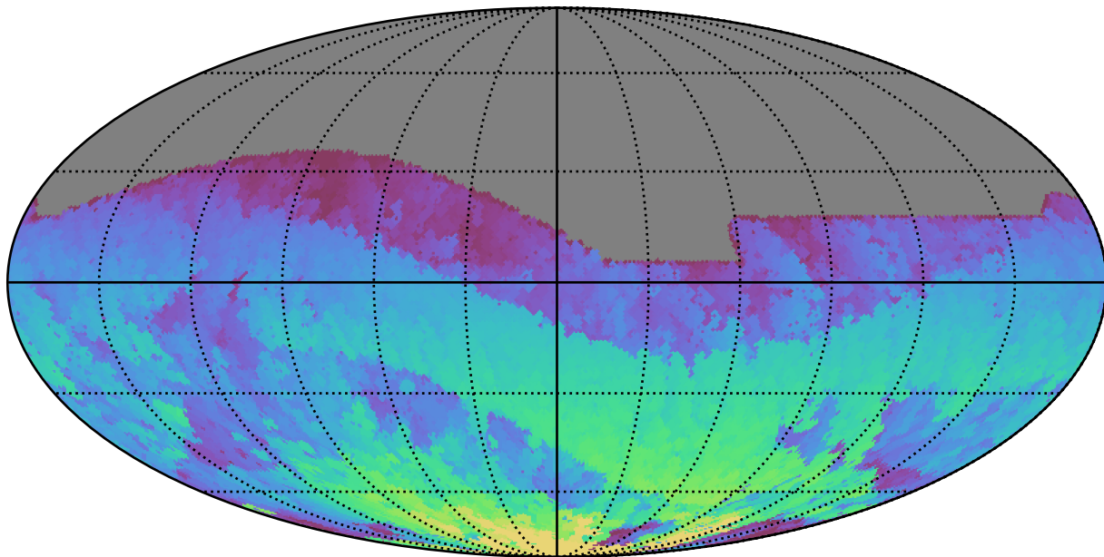
noroll_mjdp60_v3.4_10yrs All sky z band: Max HA
