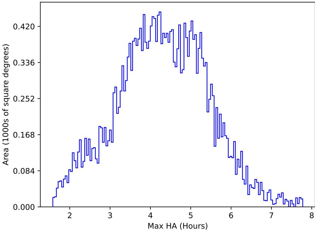
noroll_mjdp60_v3.4_10yrs All sky z band: Max HA
