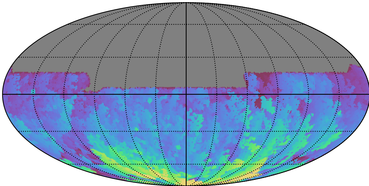
noroll_mjdp60_v3.4_10yrs All sky u band: Max HA
