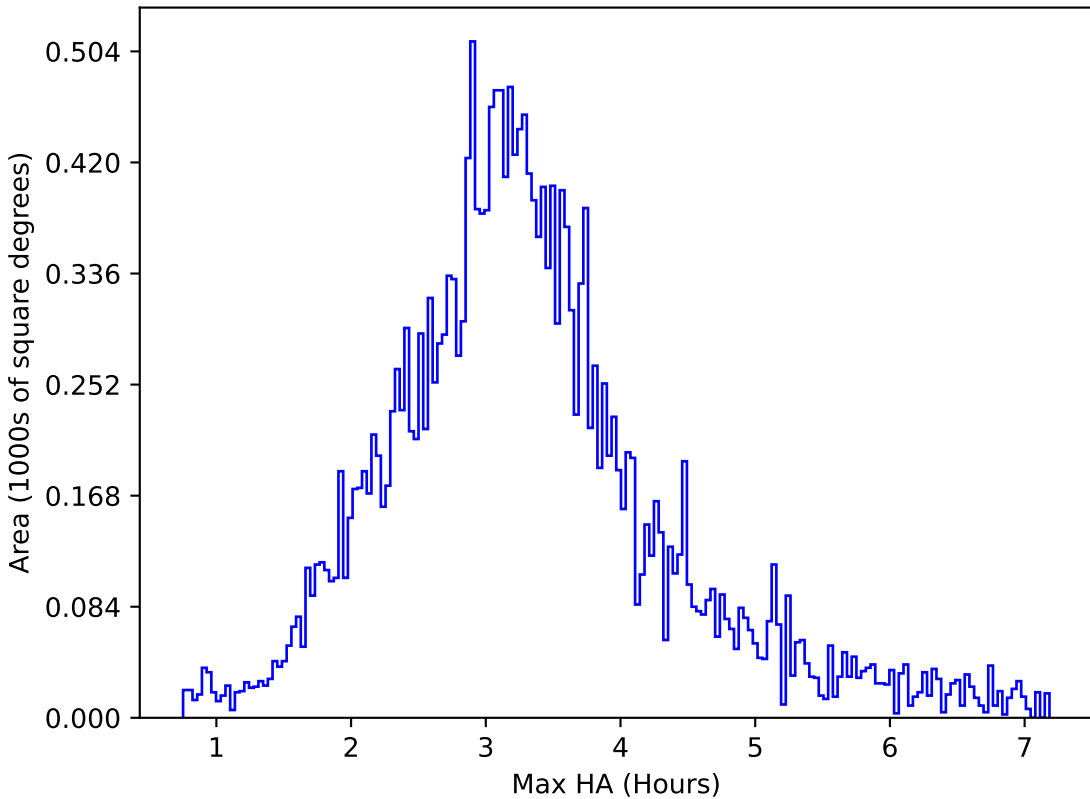
noroll_mjdp60_v3.4_10yrs All sky u band: Max HA
