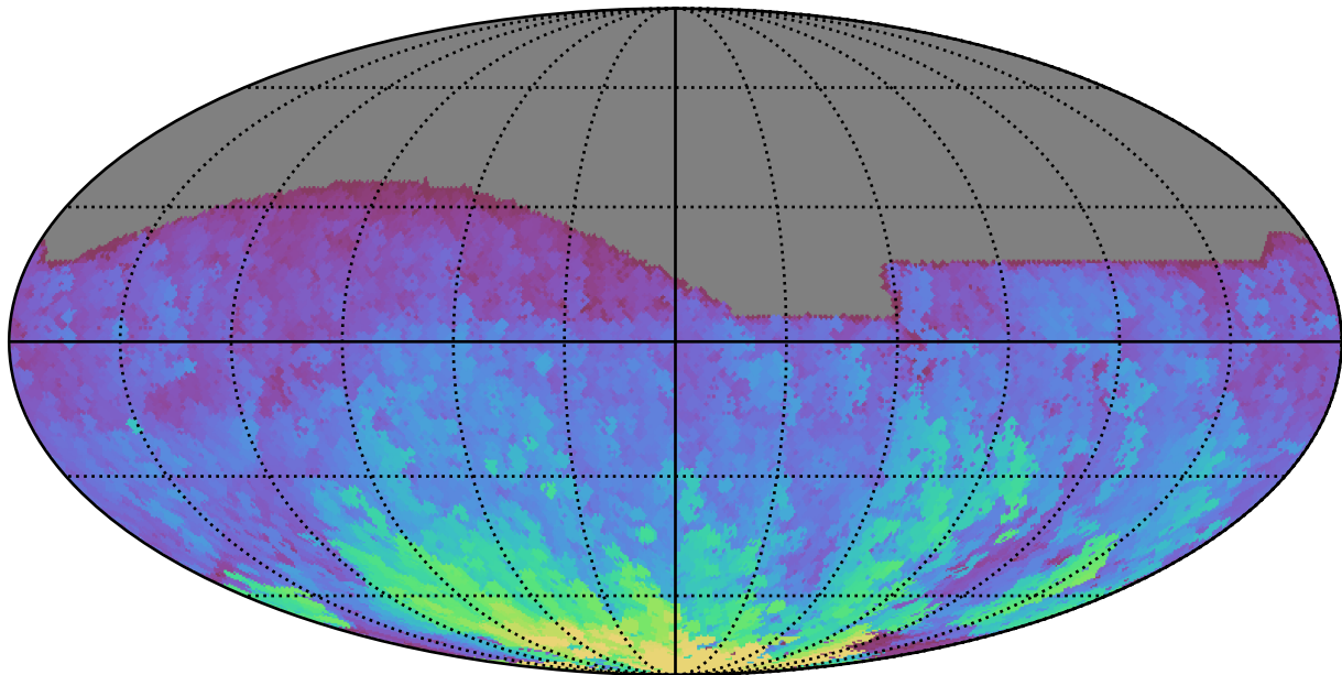
noroll_mjdp60_v3.4_10yrs All sky r band: Max HA
