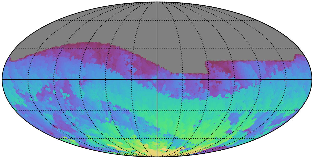
noroll_mjdp60_v3.4_10yrs All sky i band: Max HA
