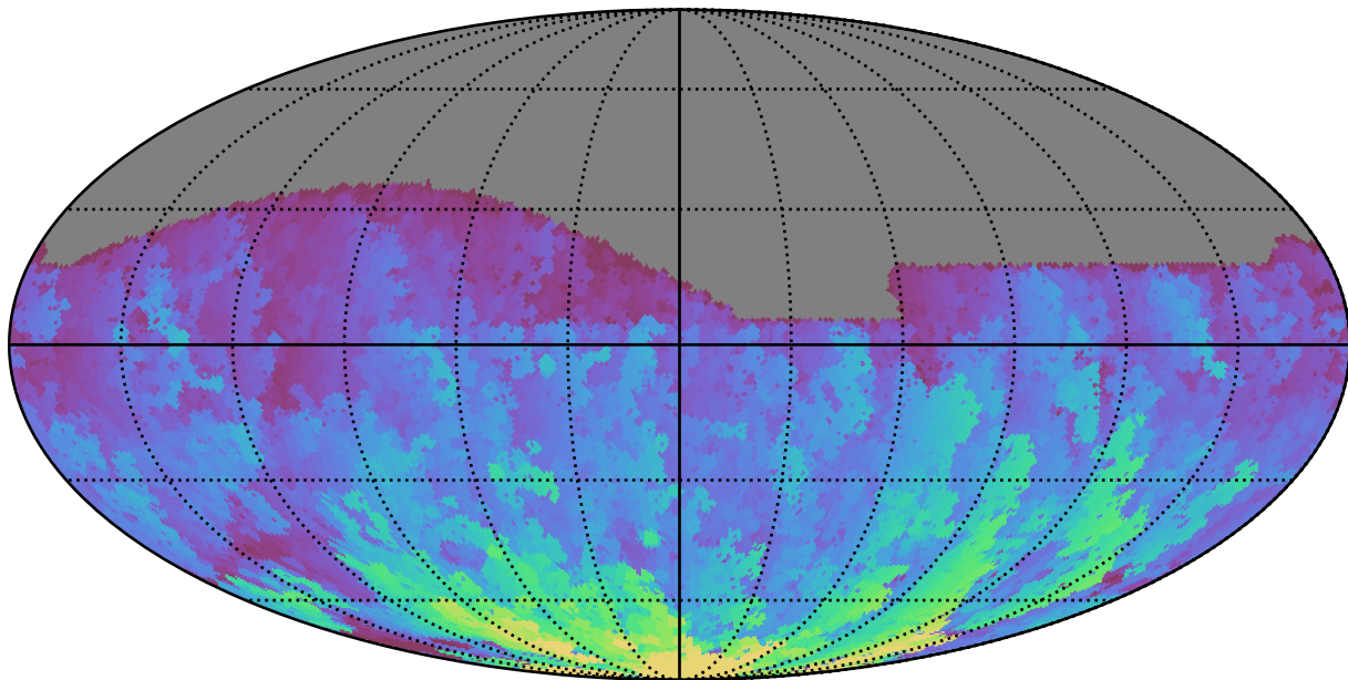
noroll_mjdp60_v3.4_10yrs All sky g band: Max HA
