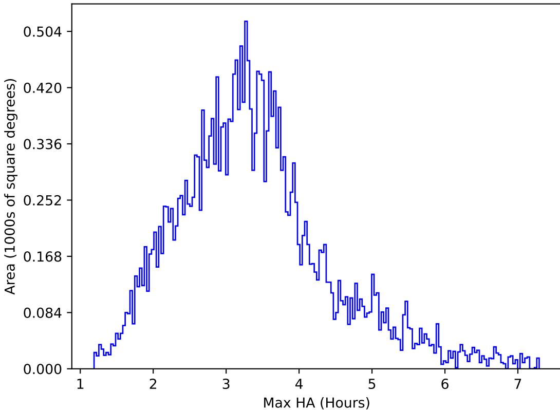
noroll_mjdp60_v3.4_10yrs All sky g band: Max HA
