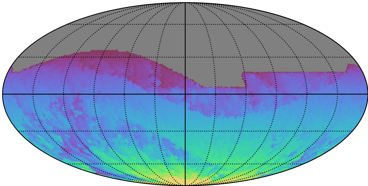
noroll_mjdp60_v3.4_10yrs All sky all bands: Max HA
