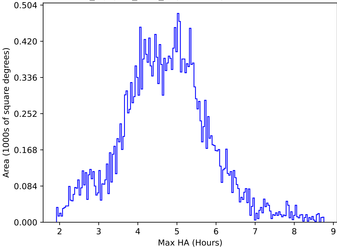
noroll_mjdp60_v3.4_10yrs All sky all bands: Max HA
