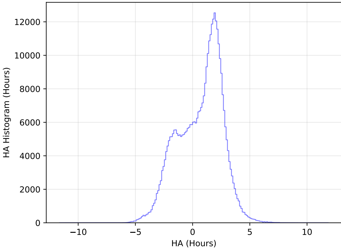
noroll_mjdp60_v3.4_10yrs WFD y band: HA Histogram
