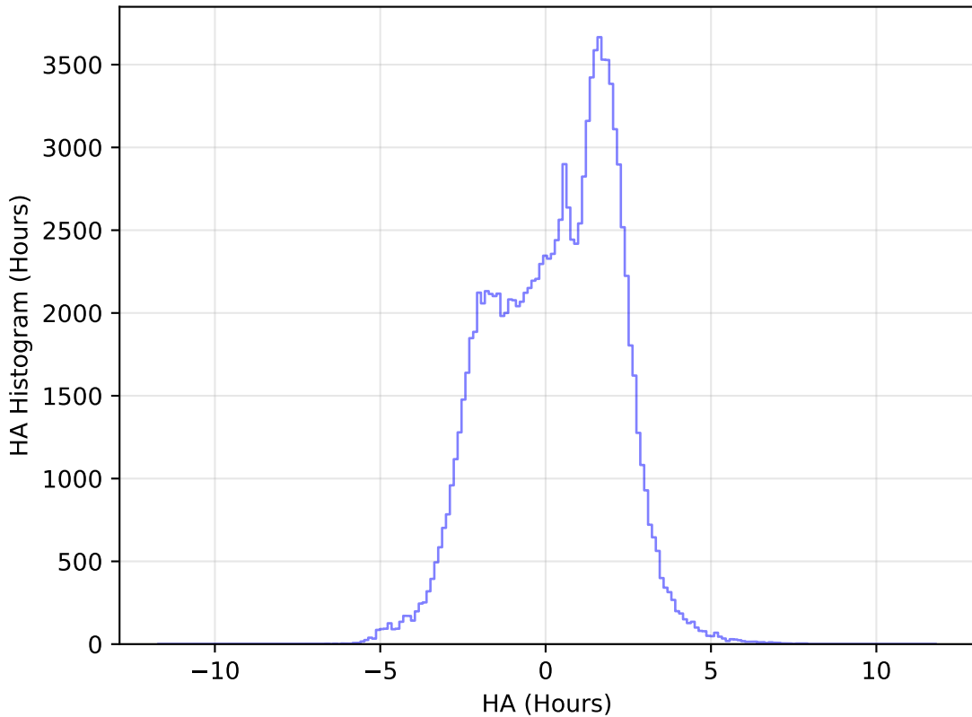
noroll_mjdp60_v3.4_10yrs WFD u band: HA Histogram
