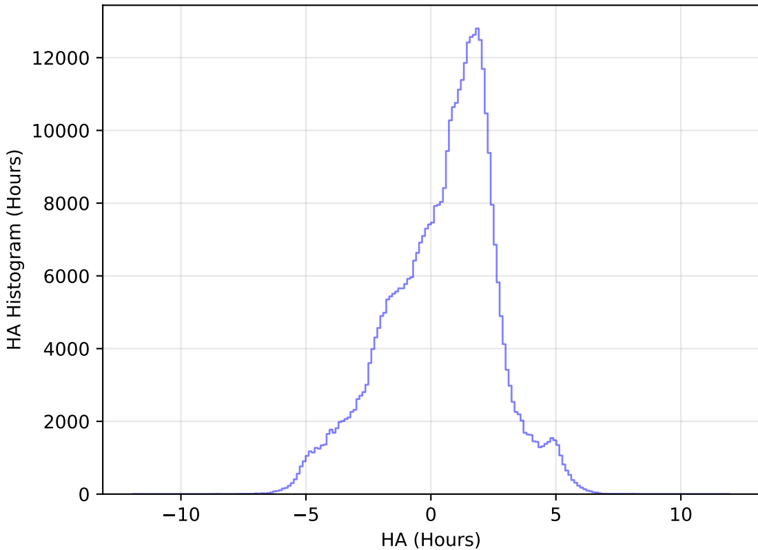
noroll_mjdp60_v3.4_10yrs All sky z band: HA Histogram
