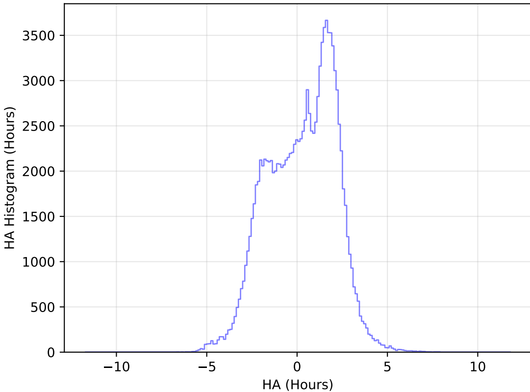
noroll_mjdp60_v3.4_10yrs All sky u band: HA Histogram
