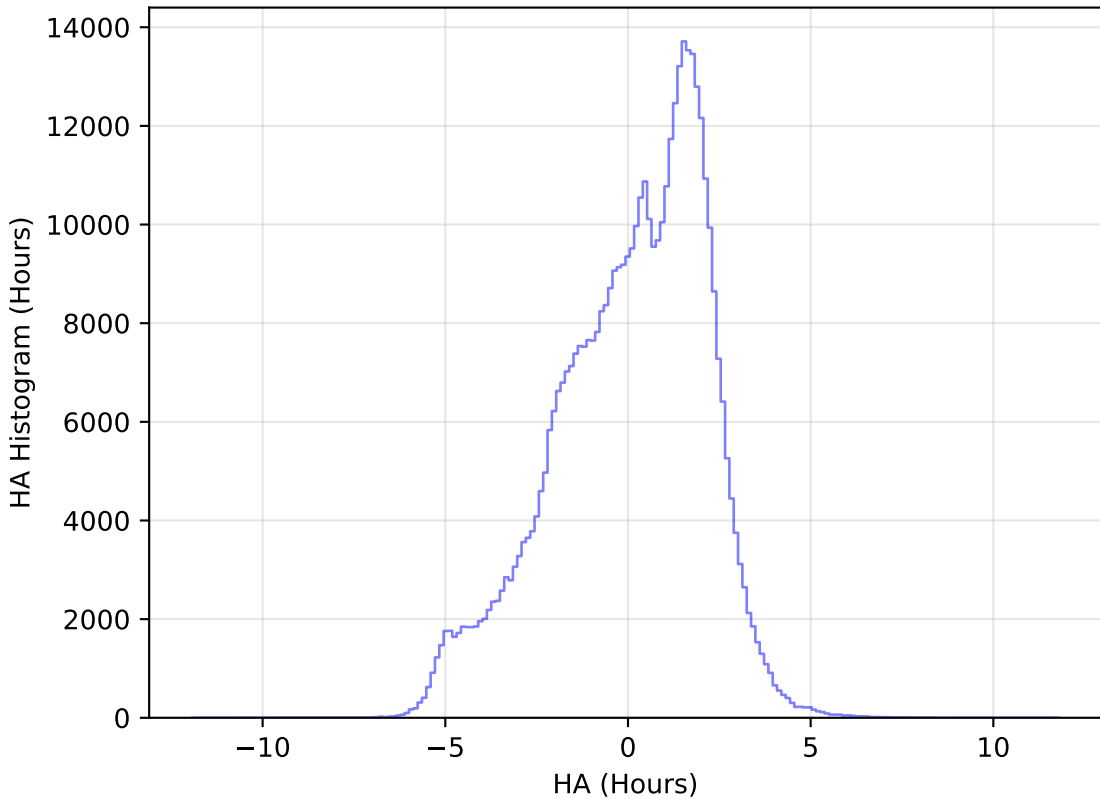
noroll_mjdp60_v3.4_10yrs All sky r band: HA Histogram
