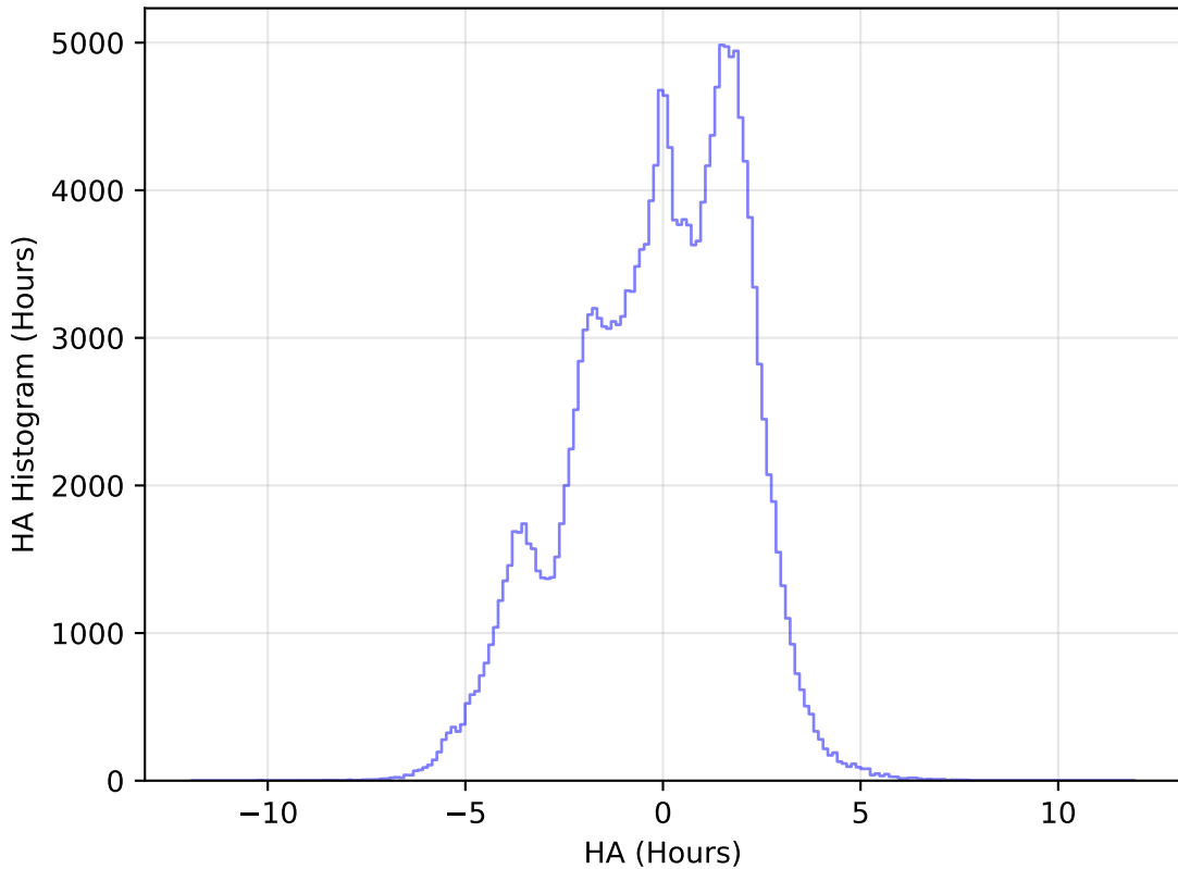
noroll_mjdp60_v3.4_10yrs All sky g band: HA Histogram
