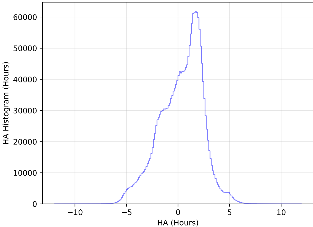
noroll_mjdp60_v3.4_10yrs All sky all bands: HA Histogram
