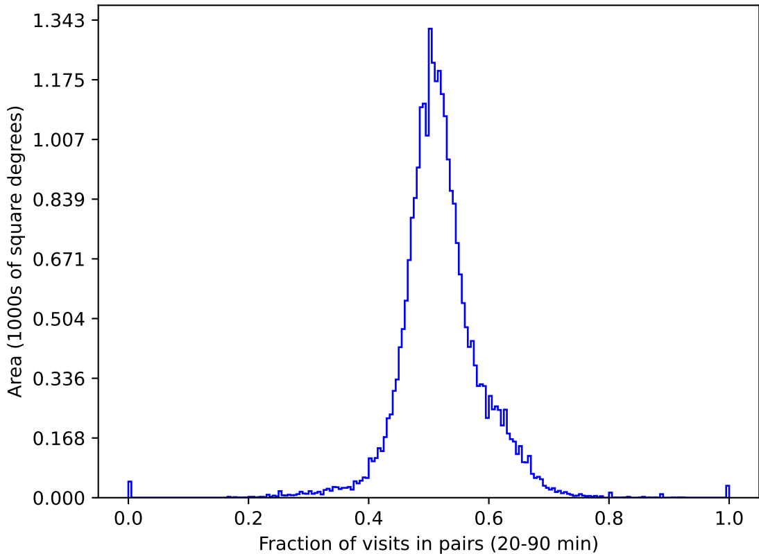
noroll_mjdp60_v3.4_10yrs gri All sky: Fraction of visits in pairs (20-90 min)
