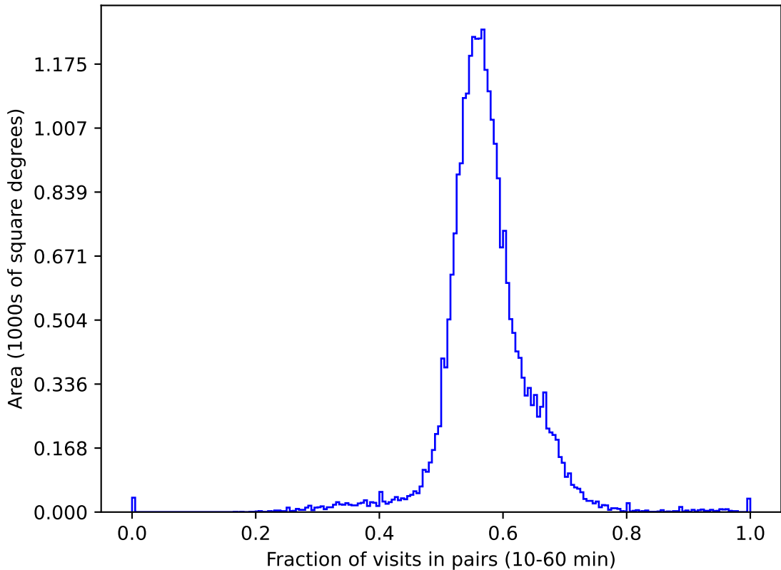
noroll_mjdp60_v3.4_10yrs gri All sky: Fraction of visits in pairs (10-60 min)
