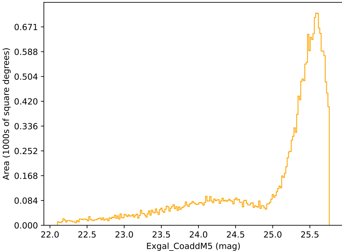
noroll_mjdp60_v3.4_10yrs Yr 3-4 r band: Exgal_CoaddM5
