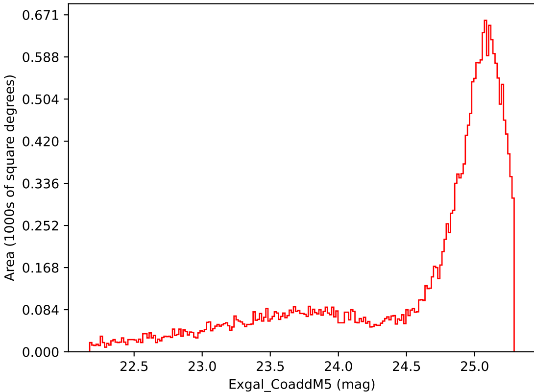
noroll_mjdp60_v3.4_10yrs Yr 3-4 i band: Exgal_CoaddM5
