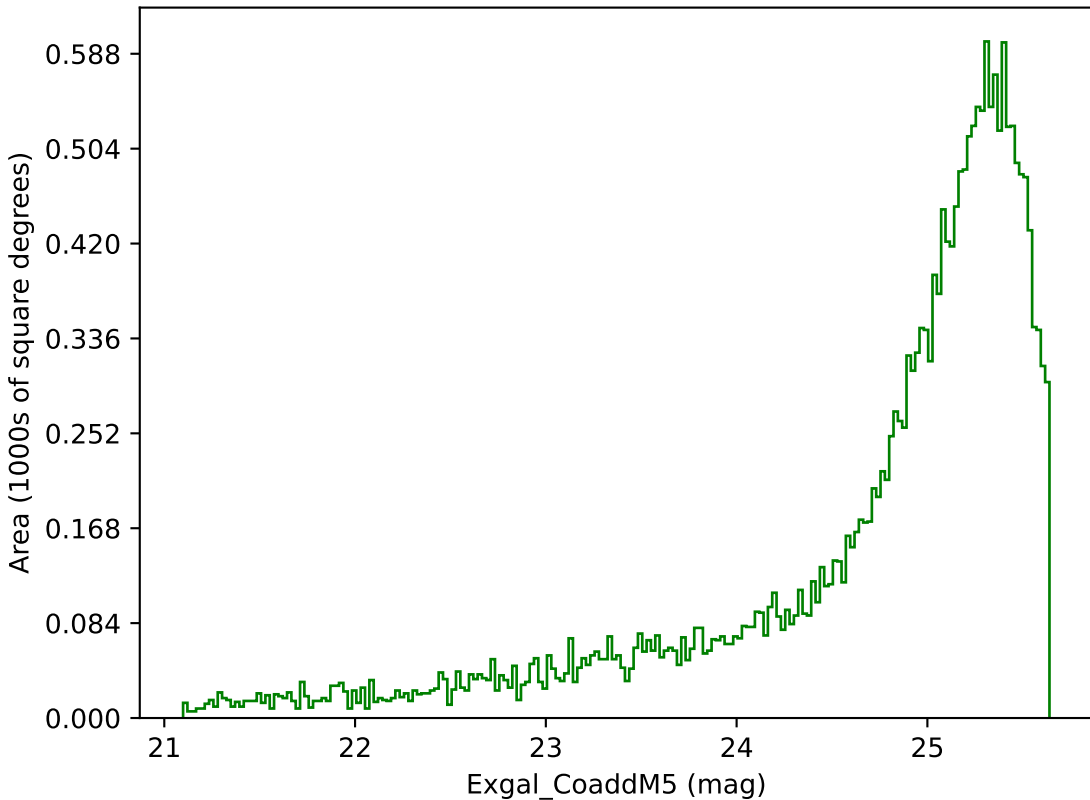
noroll_mjdp60_v3.4_10yrs Yr 3-4 g band: Exgal_CoaddM5
