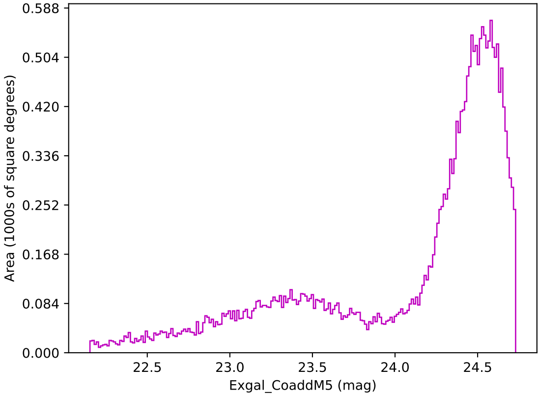
noroll_mjdp60_v3.4_10yrs Yr 1 z band: Exgal_CoaddM5
