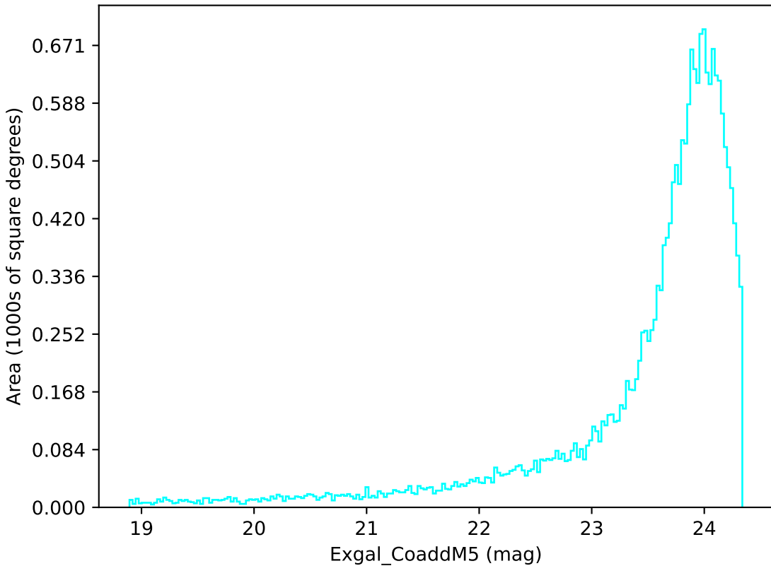
noroll_mjdp60_v3.4_10yrs Yr 1 u band: Exgal_CoaddM5
