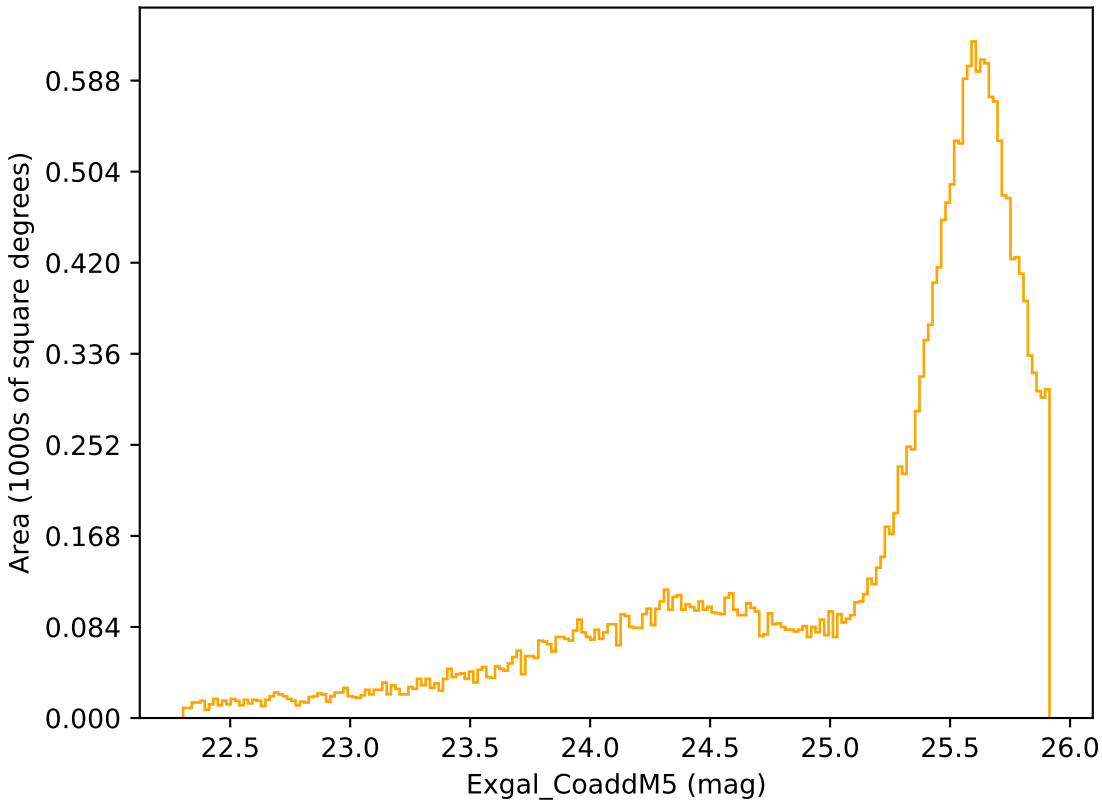
noroll_mjdp60_v3.4_10yrs Yr 1 r band: Exgal_CoaddM5
