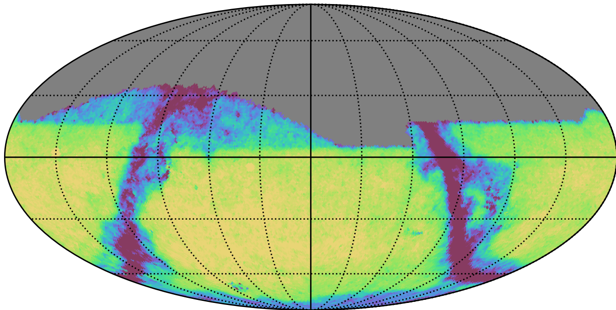
noroll_mjdp60_v3.4_10yrs Yr 1 i band: Exgal_CoaddM5
