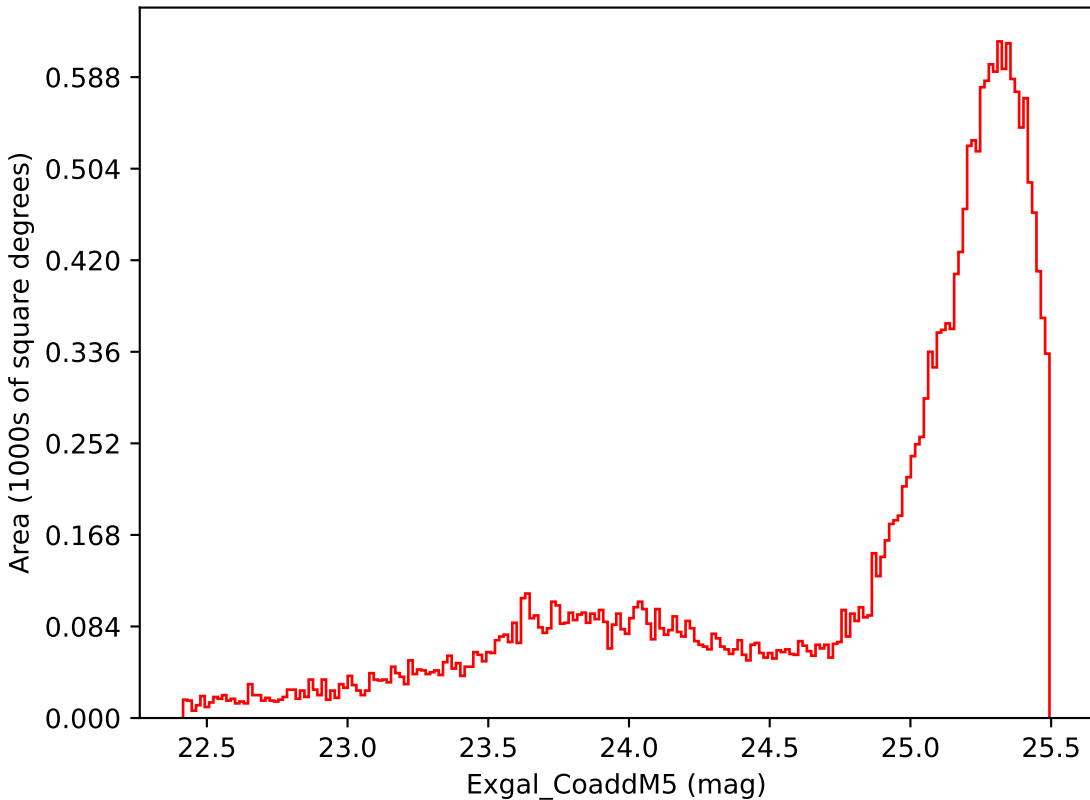
noroll_mjdp60_v3.4_10yrs Yr 1 i band: Exgal_CoaddM5
