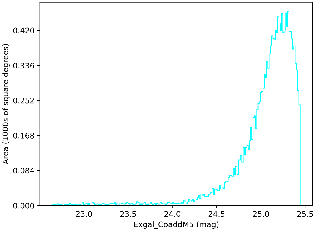
noroll_mjdp60_v3.4_10yrs WFD u band: Exgal_CoaddM5
