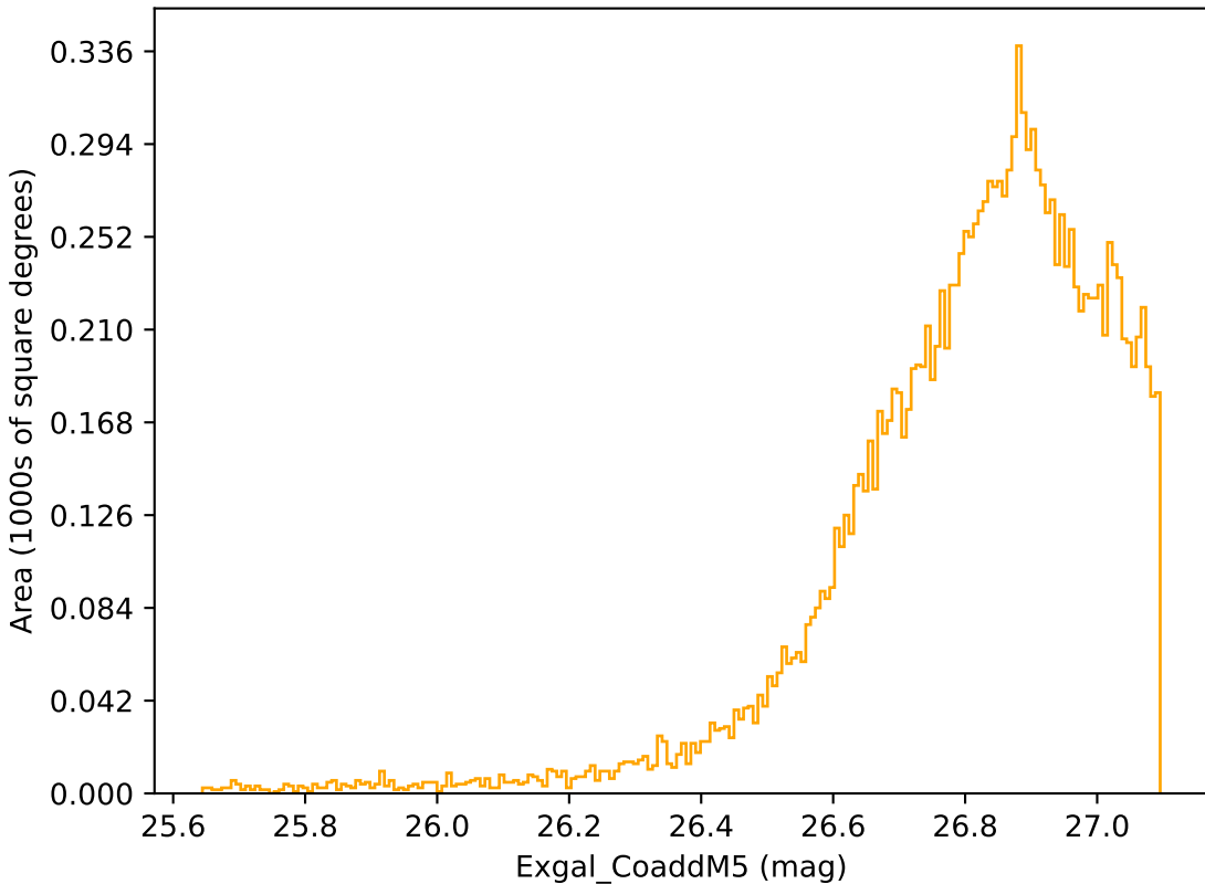
noroll_mjdp60_v3.4_10yrs WFD r band: Exgal_CoaddM5
