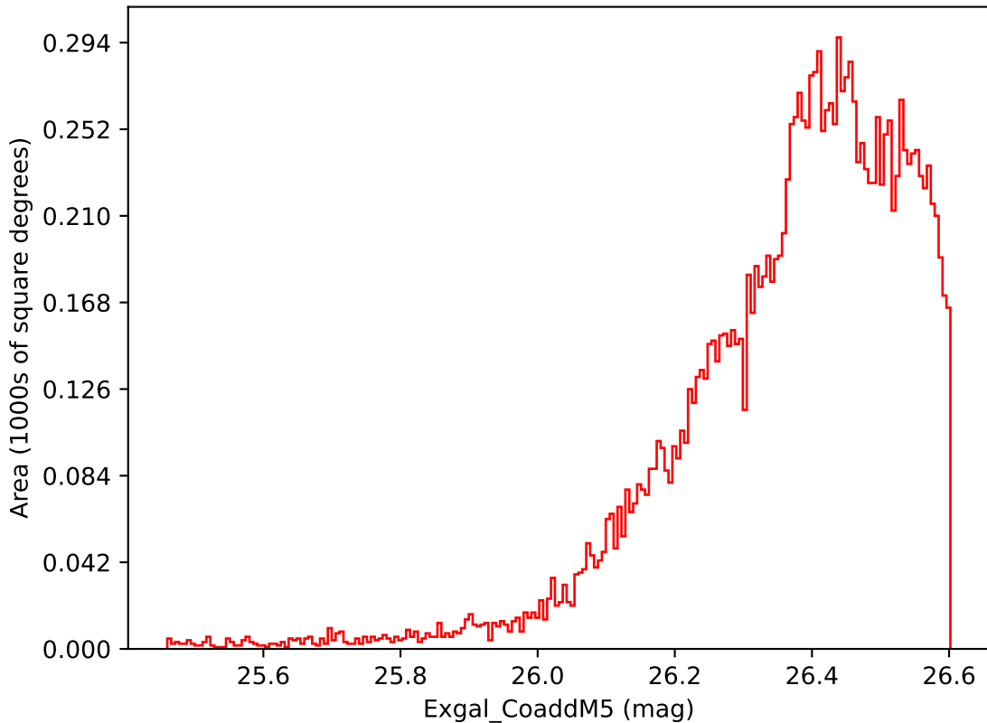
noroll_mjdp60_v3.4_10yrs WFD i band: Exgal_CoaddM5
