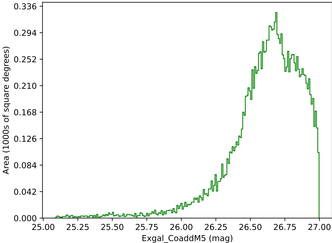
noroll_mjdp60_v3.4_10yrs WFD g band: Exgal_CoaddM5
