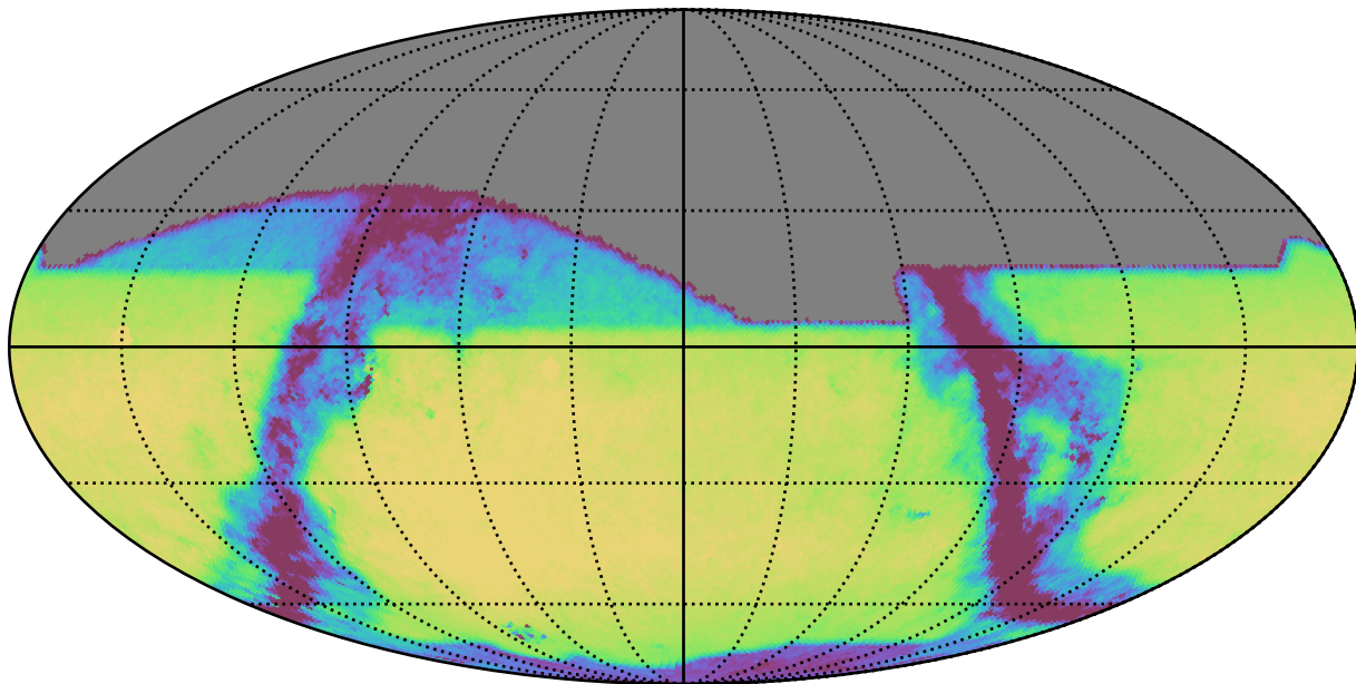
noroll_mjdp60_v3.4_10yrs All sky z band: Exgal_CoaddM5
