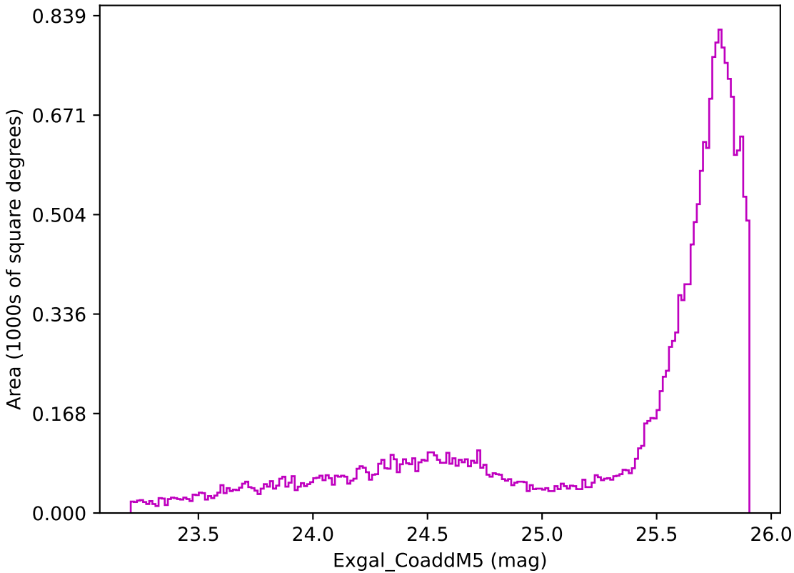
noroll_mjdp60_v3.4_10yrs All sky z band: Exgal_CoaddM5
