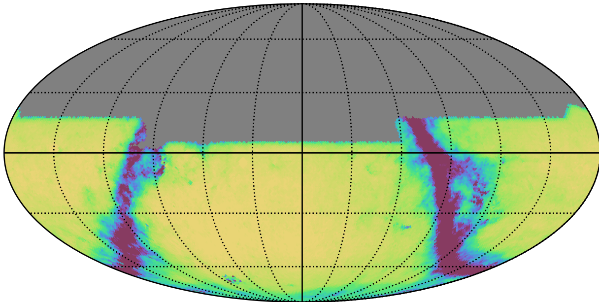
noroll_mjdp60_v3.4_10yrs All sky u band: Exgal_CoaddM5
