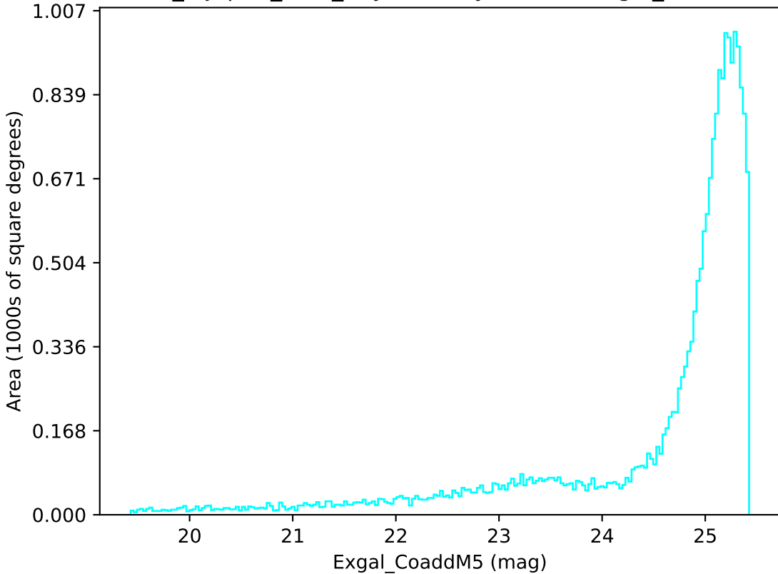
noroll_mjdp60_v3.4_10yrs All sky u band: Exgal_CoaddM5
