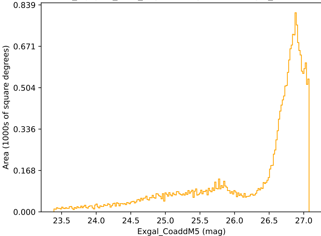
noroll_mjdp60_v3.4_10yrs All sky r band: Exgal_CoaddM5
