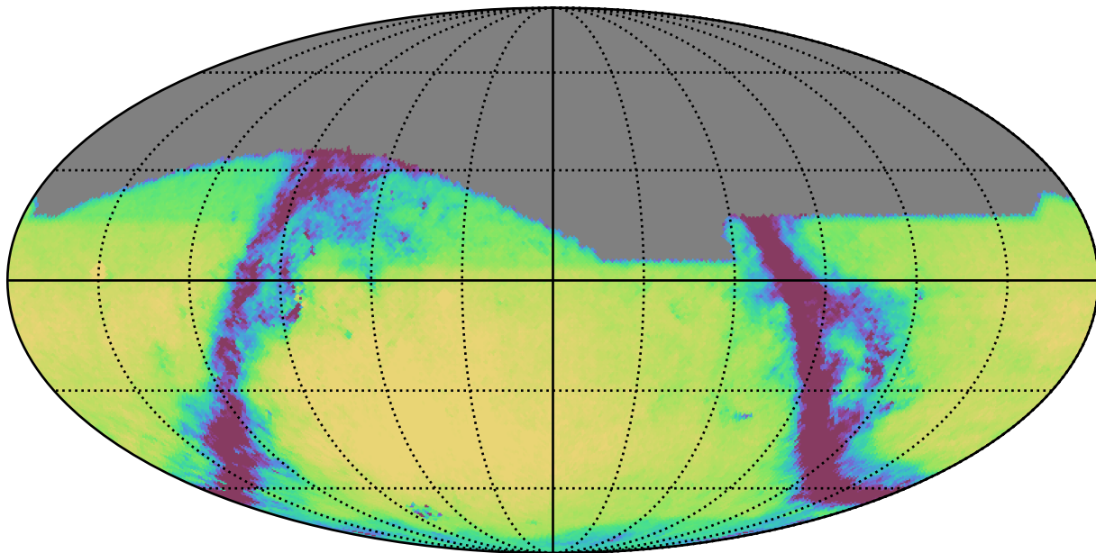
noroll_mjdp60_v3.4_10yrs All sky g band: Exgal_CoaddM5
