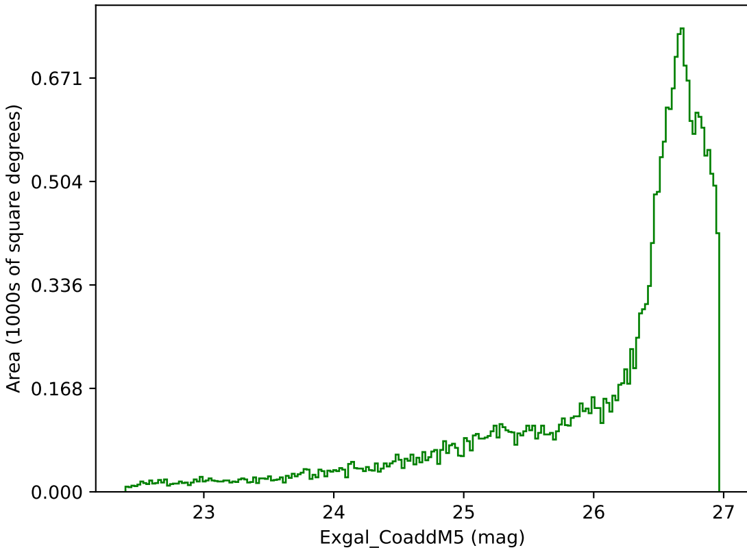
noroll_mjdp60_v3.4_10yrs All sky g band: Exgal_CoaddM5
