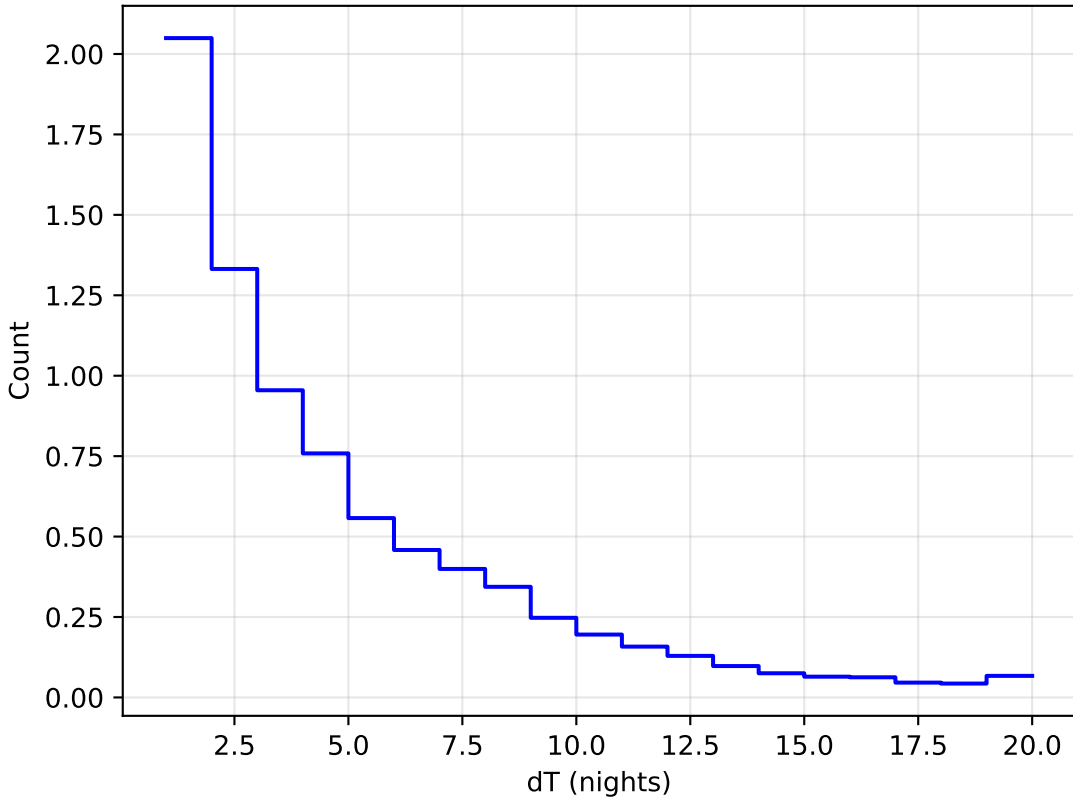
noroll_mjdp60_v3.4_10yrs WFD all bands: DeltaNight Histogram
