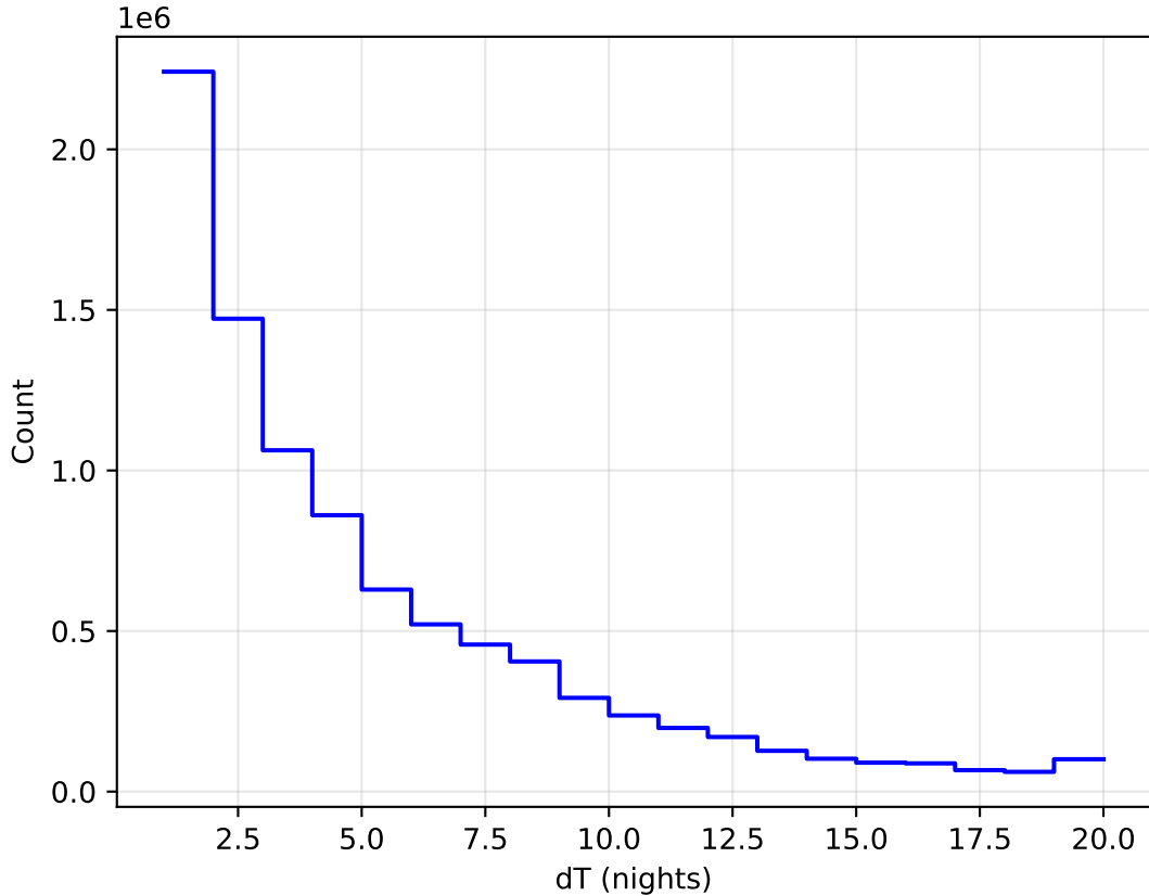
noroll_mjdp60_v3.4_10yrs All sky all bands: DeltaNight Histogram
