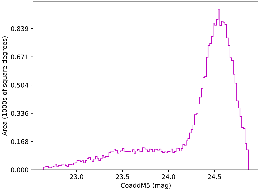
noroll_mjdp60_v3.4_10yrs Yr 3-4 z band: CoaddM5
