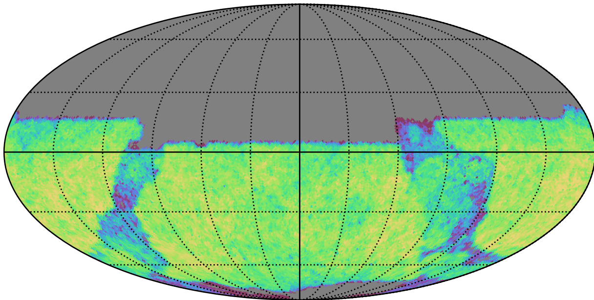
noroll_mjdp60_v3.4_10yrs Yr 3-4 y band: CoaddM5
